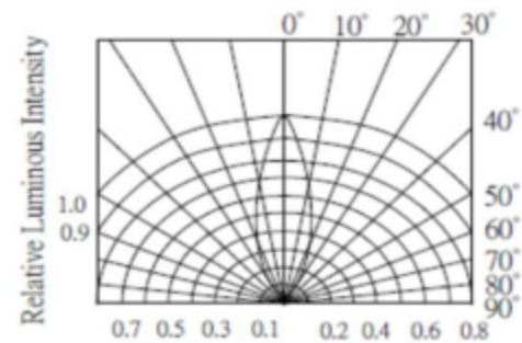
RADIATION DIAGRAM
